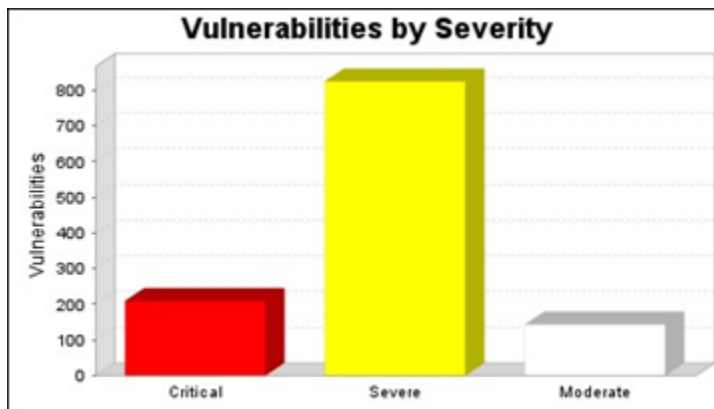
Fig 7 - Vulnerability Chart
