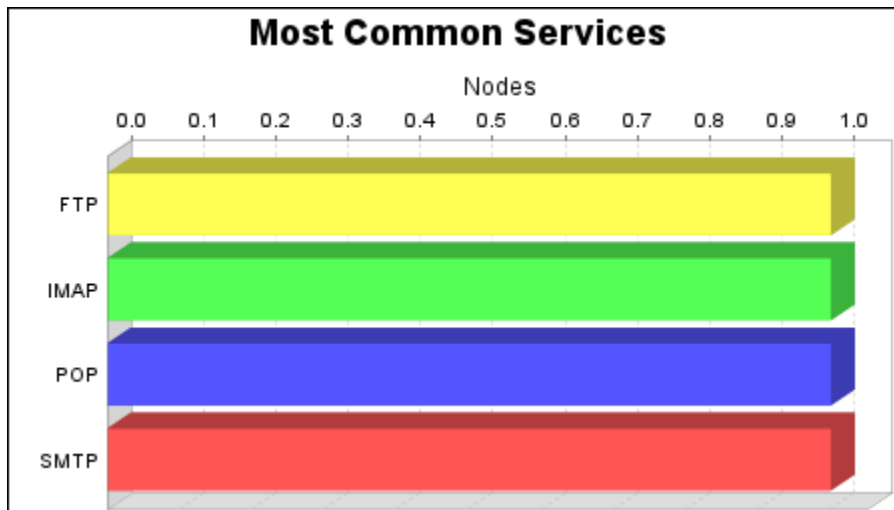
Fig 10 - Services Running
