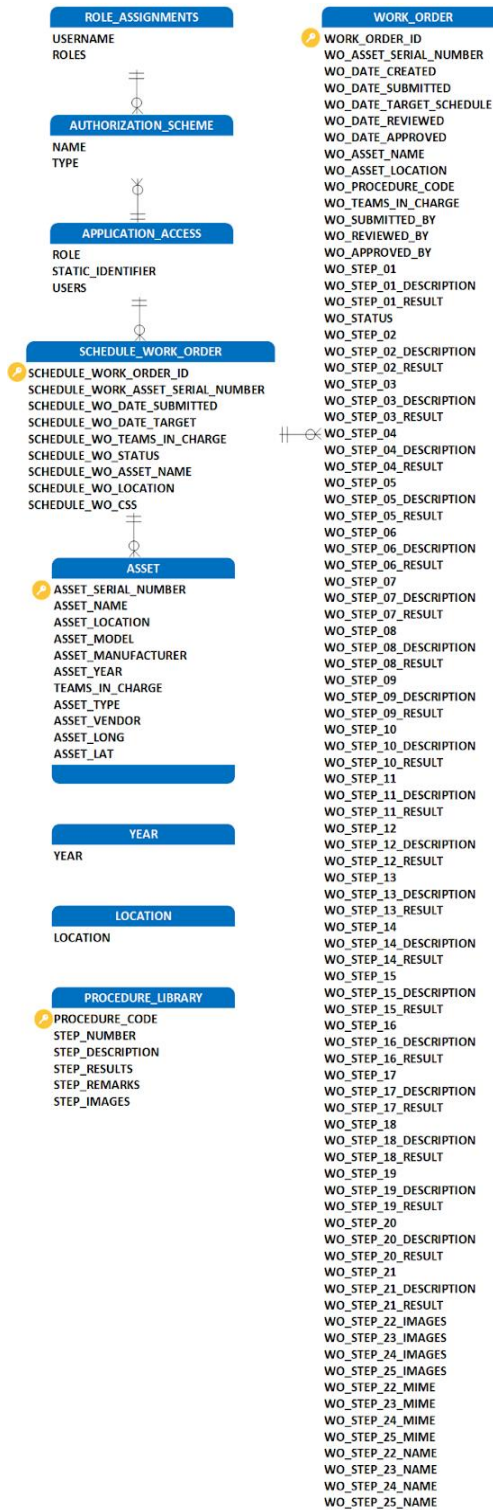
Fig 5 - Database Design
