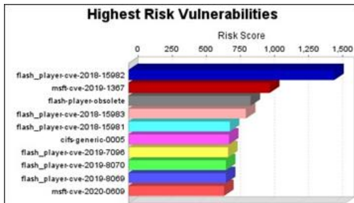
Fig 9 - Vulnerability Ranking
