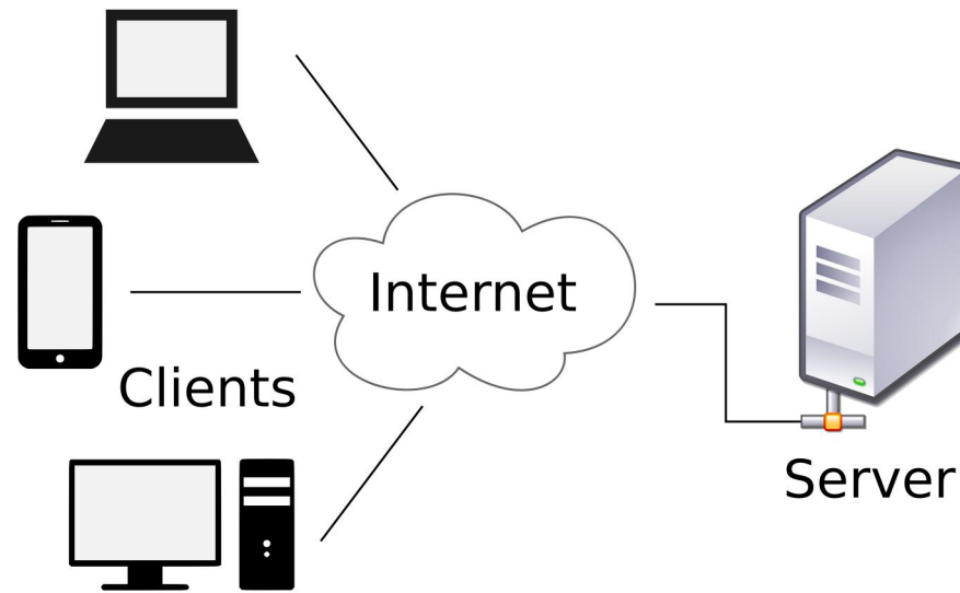
Figure 1: Client-Server model
