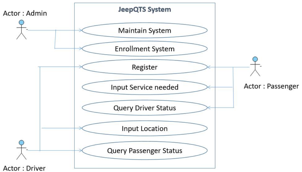
Figure 2: Use case model of JeepQ Tracking System
