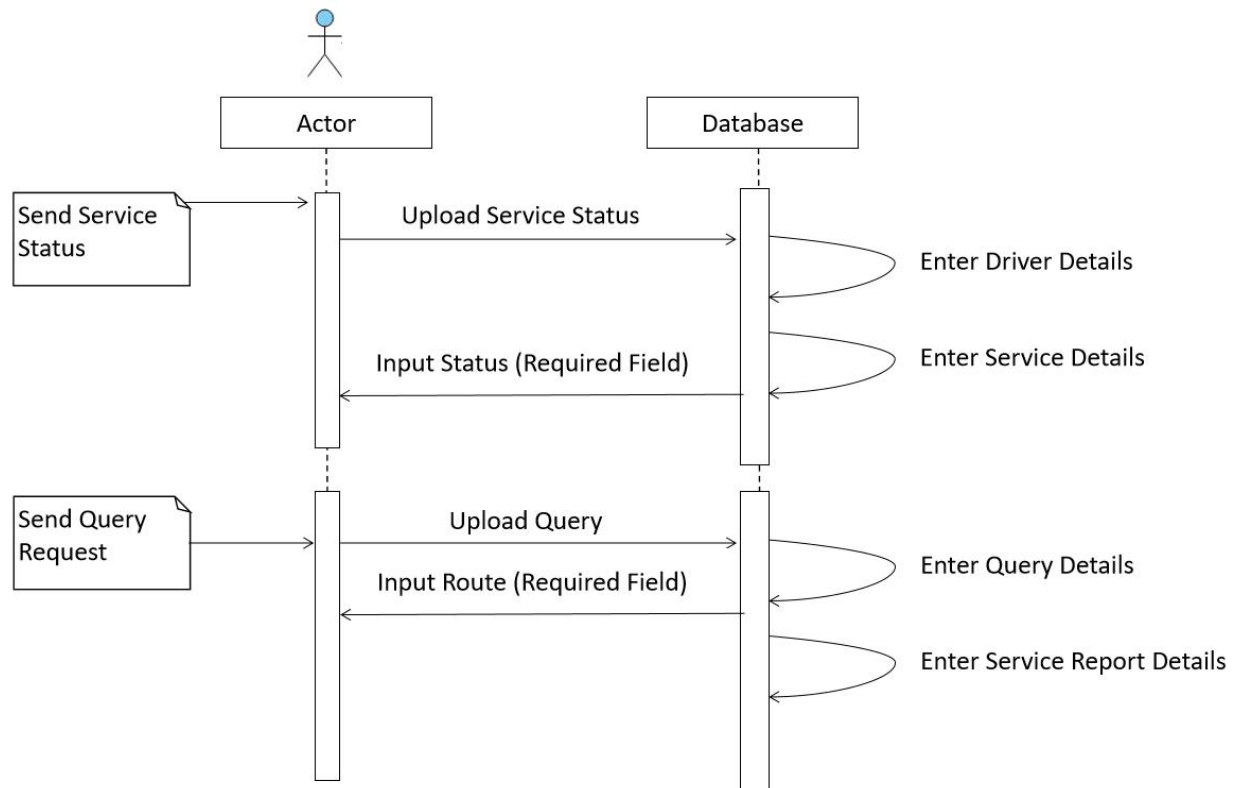
Figure 5 : Sequence diagram for Driver Upload or Query requests
