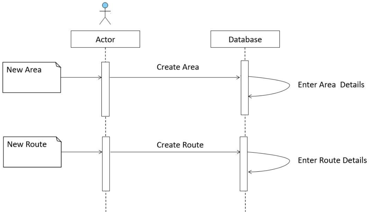
Figure 3 : Sequence diagram for creating new route and user registration as well
