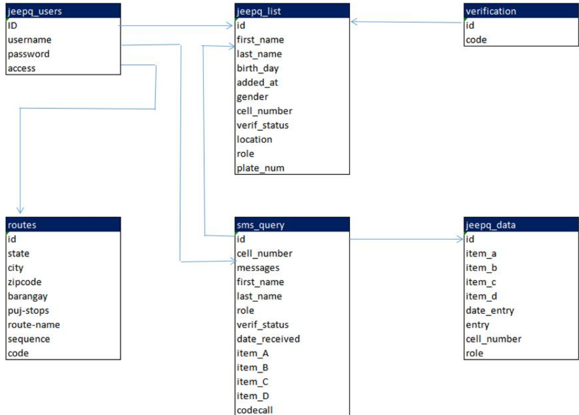
Figure 11: JeepQTS Database Model
